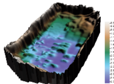
Fig 2. 3D dam model created by Discover 3D.
